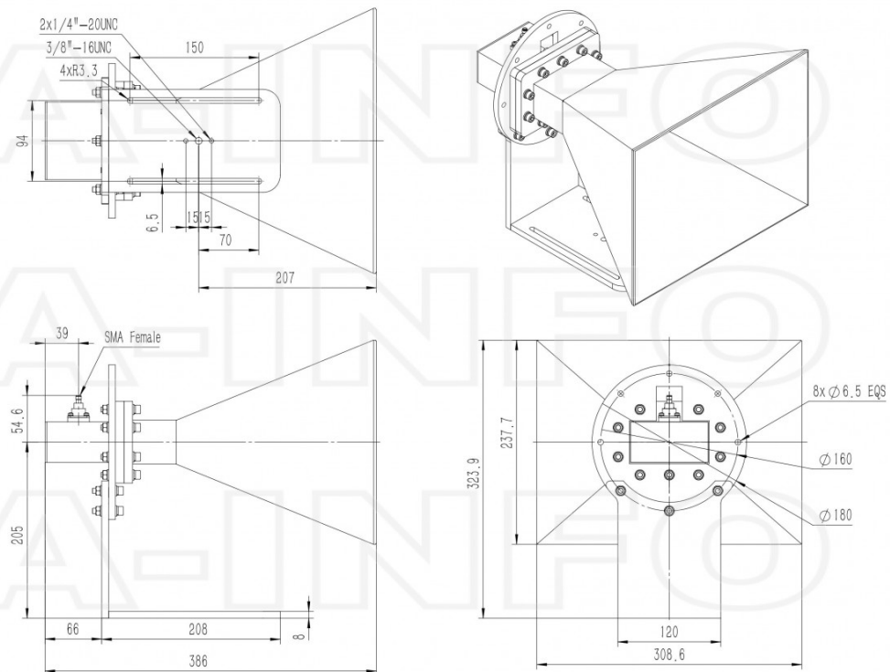
SMA Female Output with L Type Mounting Bracket (Option, P/N: LB-340-10-C-L)
